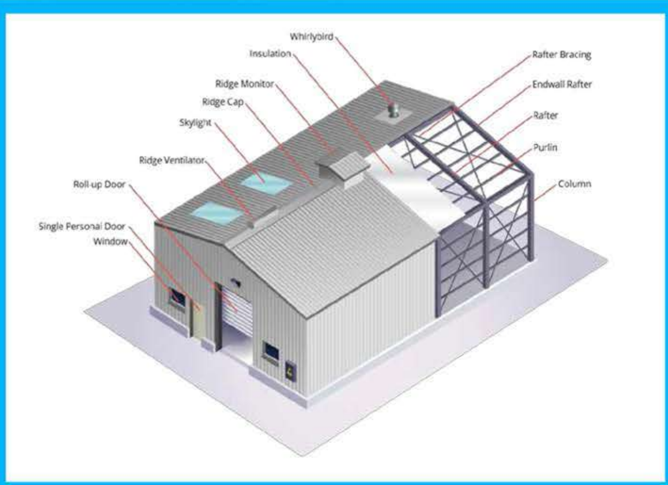
Prefabricated House
